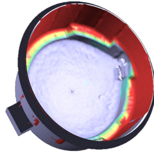
LCS' 3-D output provides quantitative and qualitative assessment of vessel lining thickness, such as this EAF profile.
