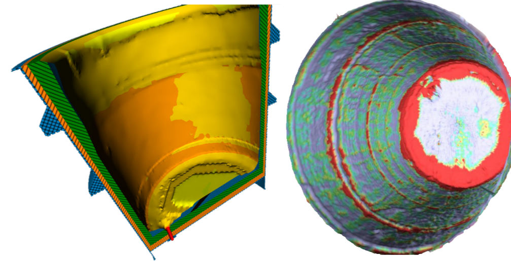
3-D Contour of Ladle Lining Thickness Measured with LCS
